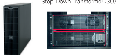
Smart-UPS RT
